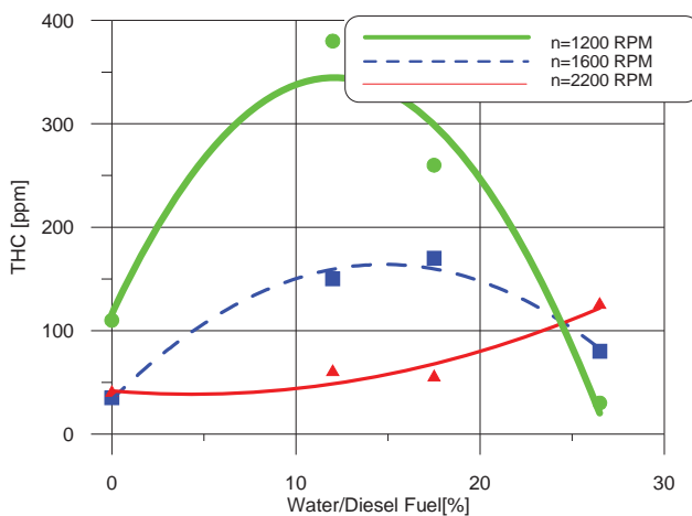
Fig. 2. Effect of water content of the fuel oil - water emulsion on the emission of unburned hydrocarbons THC
