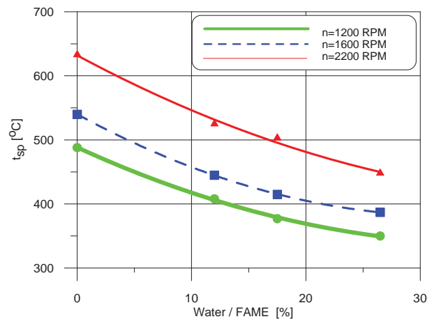
Fig. 13. Effect of water content of the emulsion FAME - water on the exhaust gases temperature
