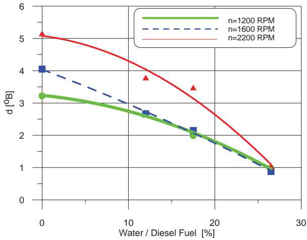
Fig. 8. Effect of water content of the fuel oil - water emulsion on the exhaust smoke - d
