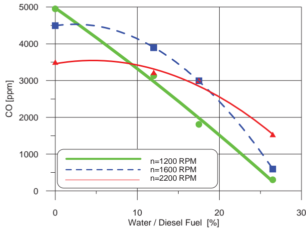
Fig. 4. Effect of water content of the fuel oil - water emulsion on the emission of carbon monoxide CO
