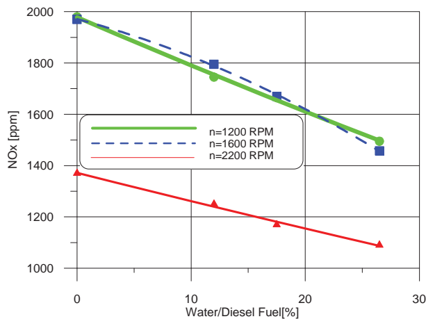
Fig. 6. Effect of water content in the fuel oil - water emulsion on the emission of NOx
