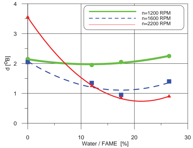
Fig. 9. Effect of water content of the emulsion FAME fuel - water on the exhaust smoke - d
