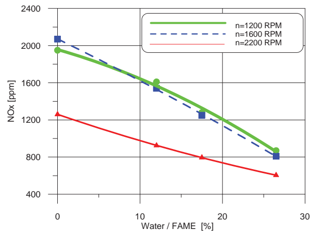
Fig. 7. Effect of water content of the FAME fuel - water emulsion on the emission of NOx
