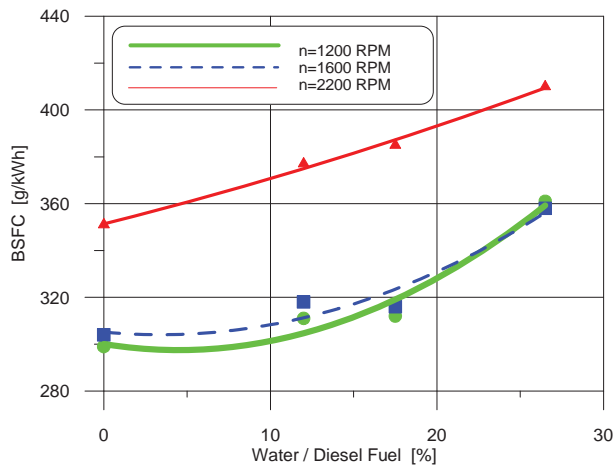
Fig. 10. Effect of water content of the fuel oil - water emulsion on specific fuel consumption - BSFC
