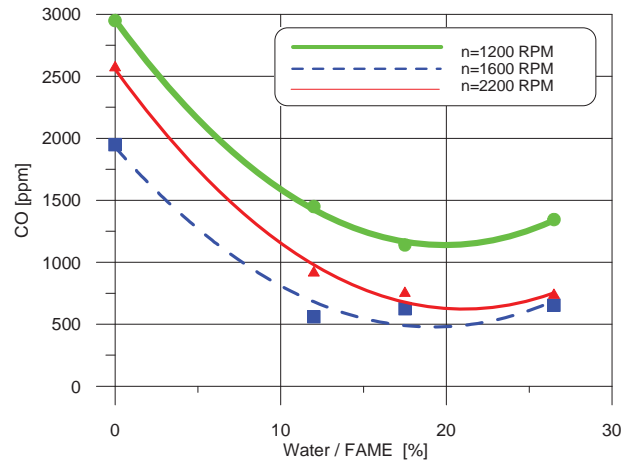
Fig. 5. Effect of water content of the emulsion FAME - water on the emission of carbon monoxide CO
