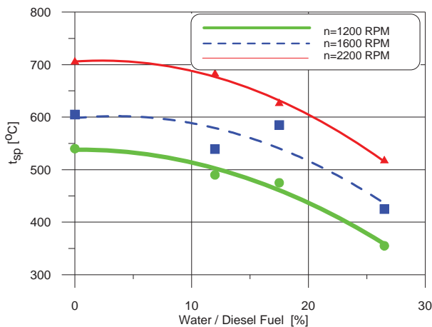
Fig. 12. Effect of water content of the fuel oil - water emulsion on the exhaust gases temperature
