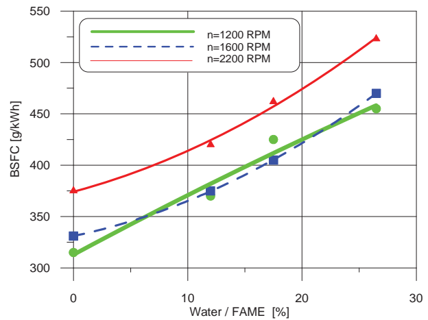
Fig. 11. Effect of water content of the FAME fuel - water emulsion on specific fuel consumption - BSFC
