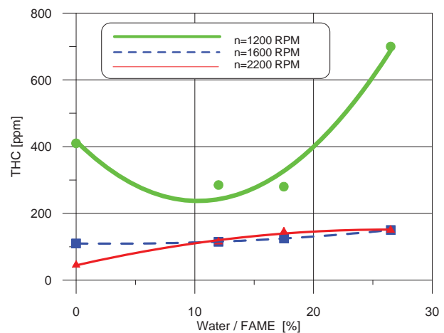
Fig. 3. Effect of water content of the FAME fuel - water emulsion on the emission of unburned hydrocarbons THC
